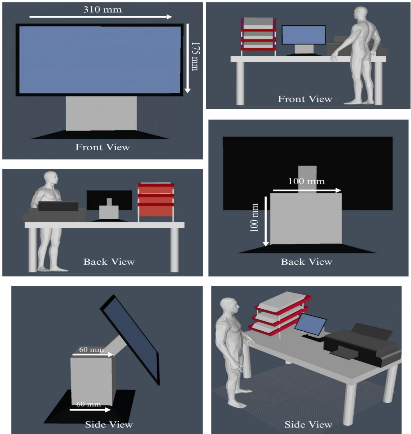
Figure 7. Perspective Plan of the Device
